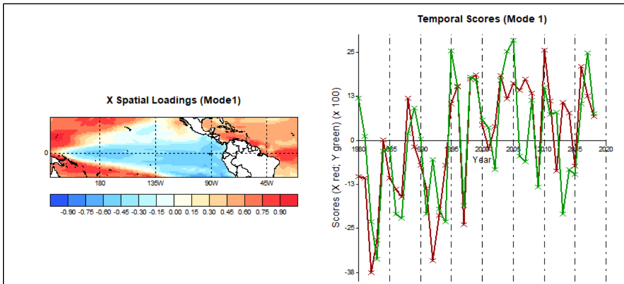
Figure 2: The X special loadings (mode 1) shows the most dominant pattern in SSTs correlation associated with above normal ACE. The canonical correlation for this pair of variables (SSTs and ACE) is over 0.69. From the temporal scores (mode 1), cool SSTs across the tropical Atlantic Ocean simultaneously with warm SSTs across the tropical Pacific
