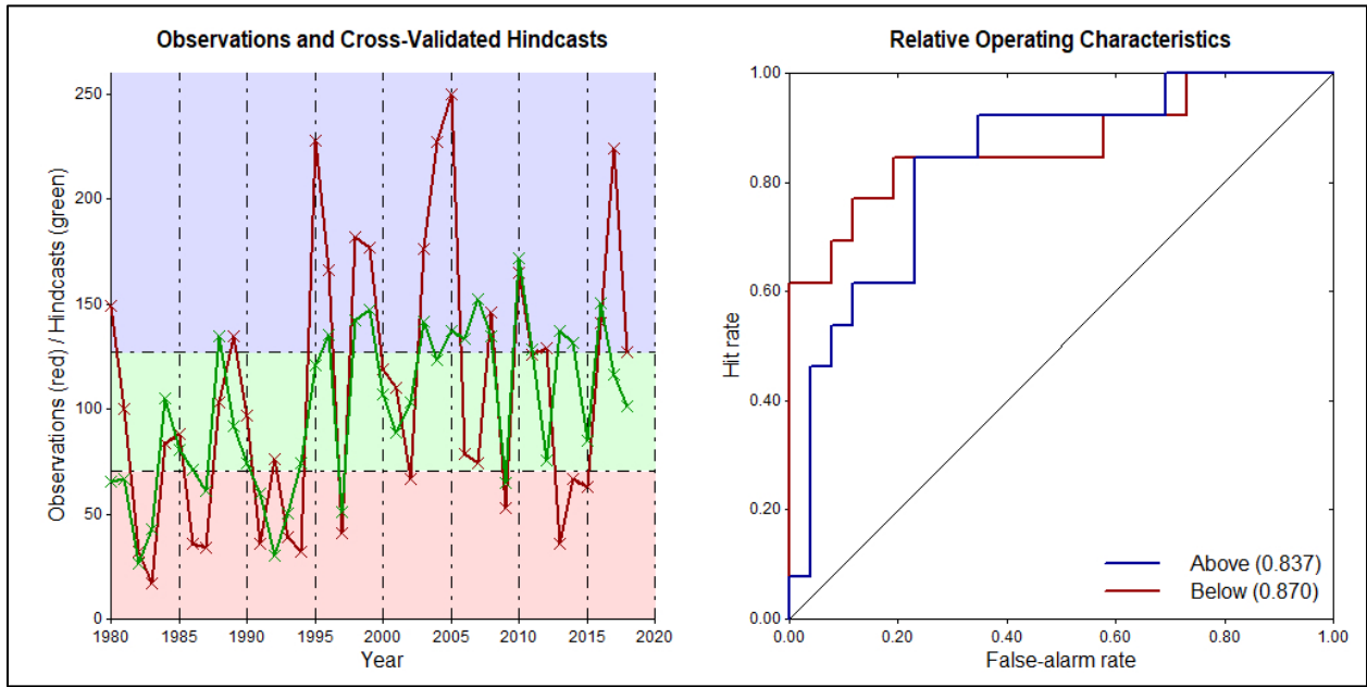
Figure 1a (left): Shows observed vs forecast ACE. The variance is a little over 36%, using GFDL-CMC22p5-FLOR_B01 mean SSTs for June to November 1982-2019, initialized May, as the training period. Figure 1b (right): The ROC diagram shows very high discrimination by the model in forecasting above and below normal ACE for the season.
