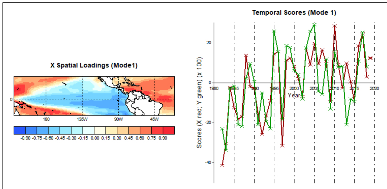
Figure 2: The X special loadings (mode 1) shows the most dominant pattern in SSTs correlation associated with above normal ACE. The canonical correlation for this pair of variables (SSTs and ACE) is over 0.79. From the temporal scores (mode 1), cool SSTs across the Pacific Ocean simultaneously with warm SSTs across the tropical Atlantic Ocean tend to coincide with above normal ACE (or season) and vice versa. Obtained using GFDL-FLOR_A02 mean SSTs for June-November 1982-2018, initialized June, as the training period.
