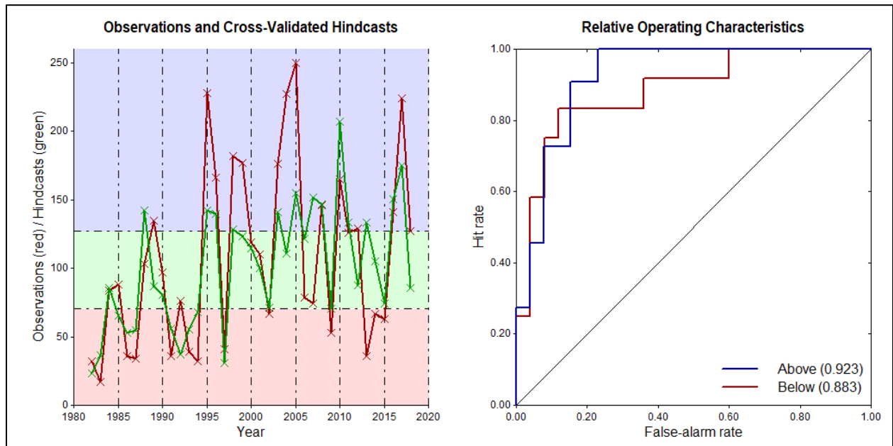
Figure 1a (left): Shows observed vs forecast ACE. The variance is over 51%, using GFDL-FLOR-A02 mean SSTs for June to November 1982-2018, initialized June, as the training period. Figure 1b (right): The ROC diagram shows very high discrimination by the model in forecasting above and below normal ACE for the season.
